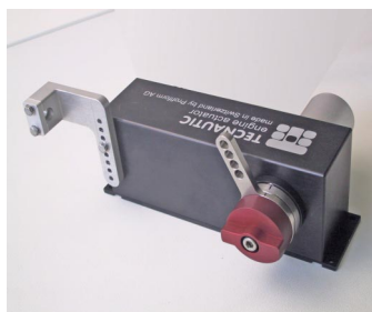
Actuator for mechanical Throttle or Shift or Water Jet Drives
